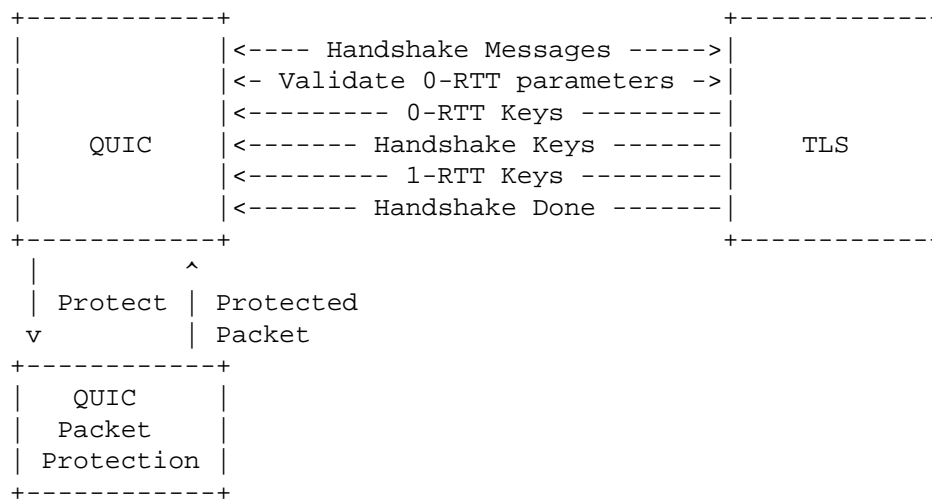
Figure 4: QUIC and TLS Interactions
